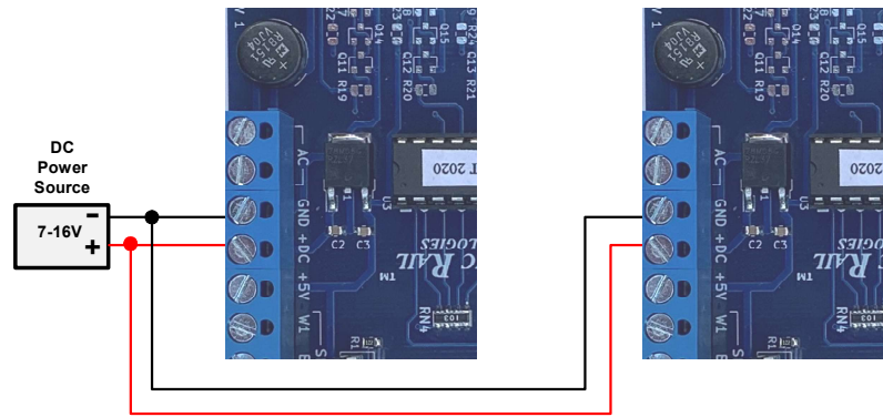
Figure 15b – DC power
