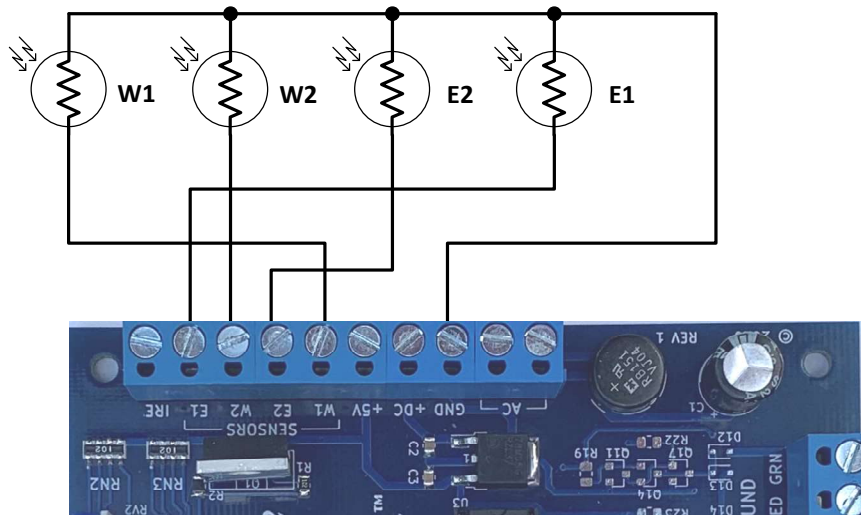
Figure 7 – Photocell wiring
