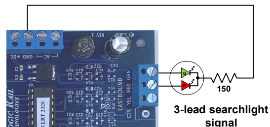
Figure 2b – three-lead bipolar (EB signal wiring shown)
