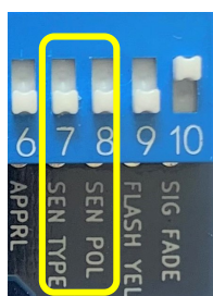
Photocell SEN TYPE – OFF SEN POL - OFF
