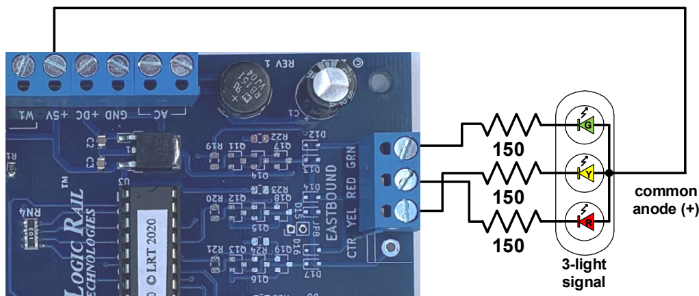
Figure 5 – 3-light signal (EB signal wiring shown)
