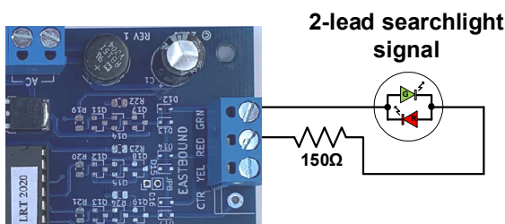
Figure 2a – two-lead bipolar (EB signal wiring shown)
