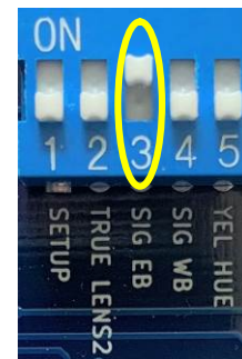
Figure 1 – selecting 2-lead or 3-lead searchlight signals (EB signal selection shown)
