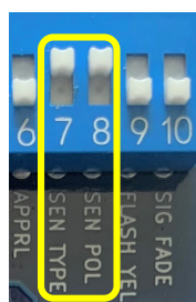
Between-the-rails Infrared SEN TYPE – ON SEN POL - ON
