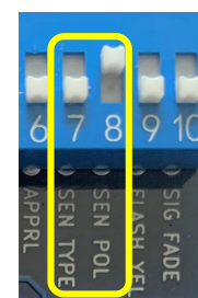
External Detector SEN TYPE – OFF SEN POL - ON
