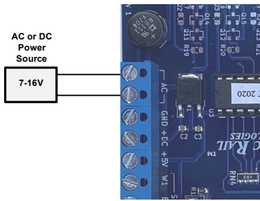
Figure 15a – AC power
