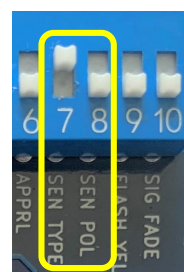
Across-the-rails Infrared SEN TYPE – ON SEN POL - OFF
