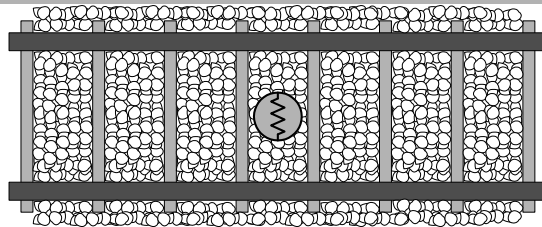
Figure 6 – photocell placement
